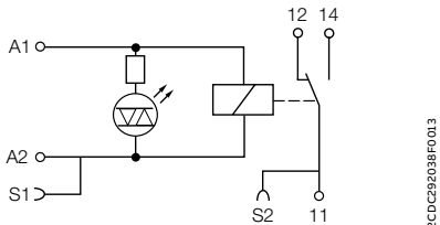
RB(R)121-12VDC/24VDC
