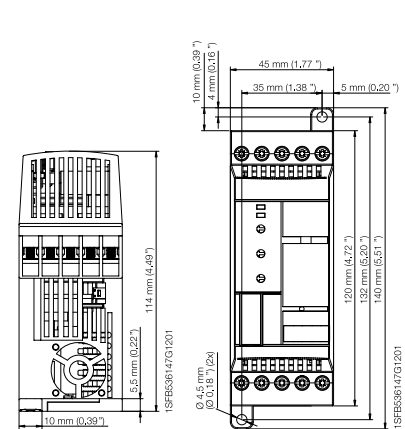
PSR3 ... PSR16
