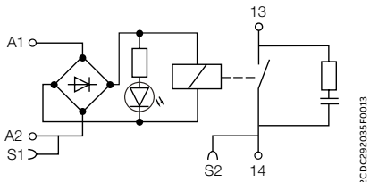
RB(R)111R-24VUC
