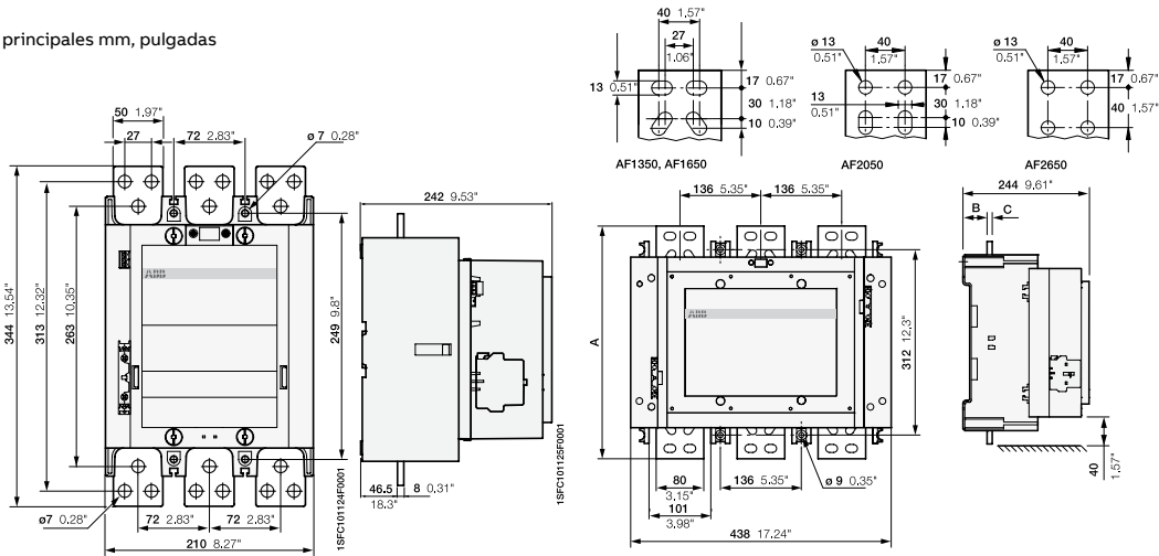
AF1350, AF1650, AF2050, AF2650, AF2850
