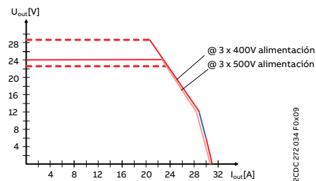
CP-T 24/20.0 Curva U/I
