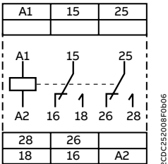
CT-WBS.22
