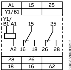
CT-MVS.23
