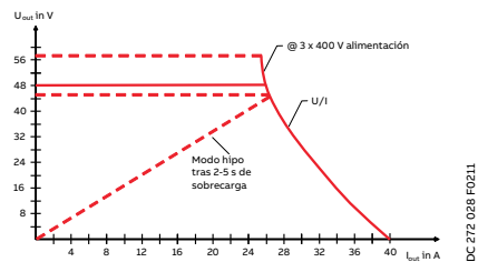
CP-T 48/20.0
