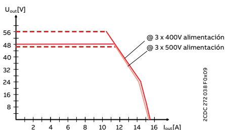
CP-T 48/10.0 Curva U/I
